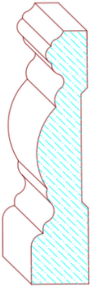
B 25 9/16" x 2 1/2"
