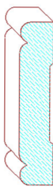
C 22 3/4" x 3"
