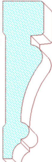
Pediment 16 1 1/2" x 5"
