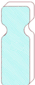
Rail 23 1 3/4" x 5"
